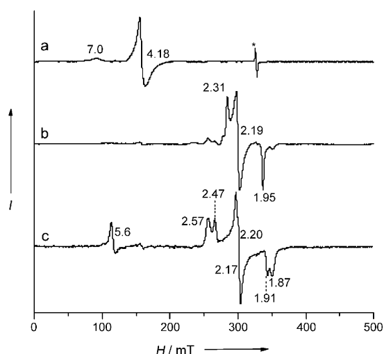
Figure 3. EPR spectra of a) complex 1 , b) 2 , and c) the room-temperature decomposition product of 2 , 77\text{ K} . The signal labeled with an asterisk originates from residual \text{O}_2^- in the solution.
